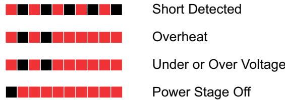
FIGURE 13. Exception or Fault Flashing Patterns
