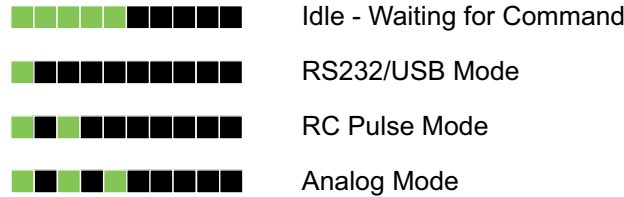
FIGURE 12. Normal Operation Flashing Patterns
